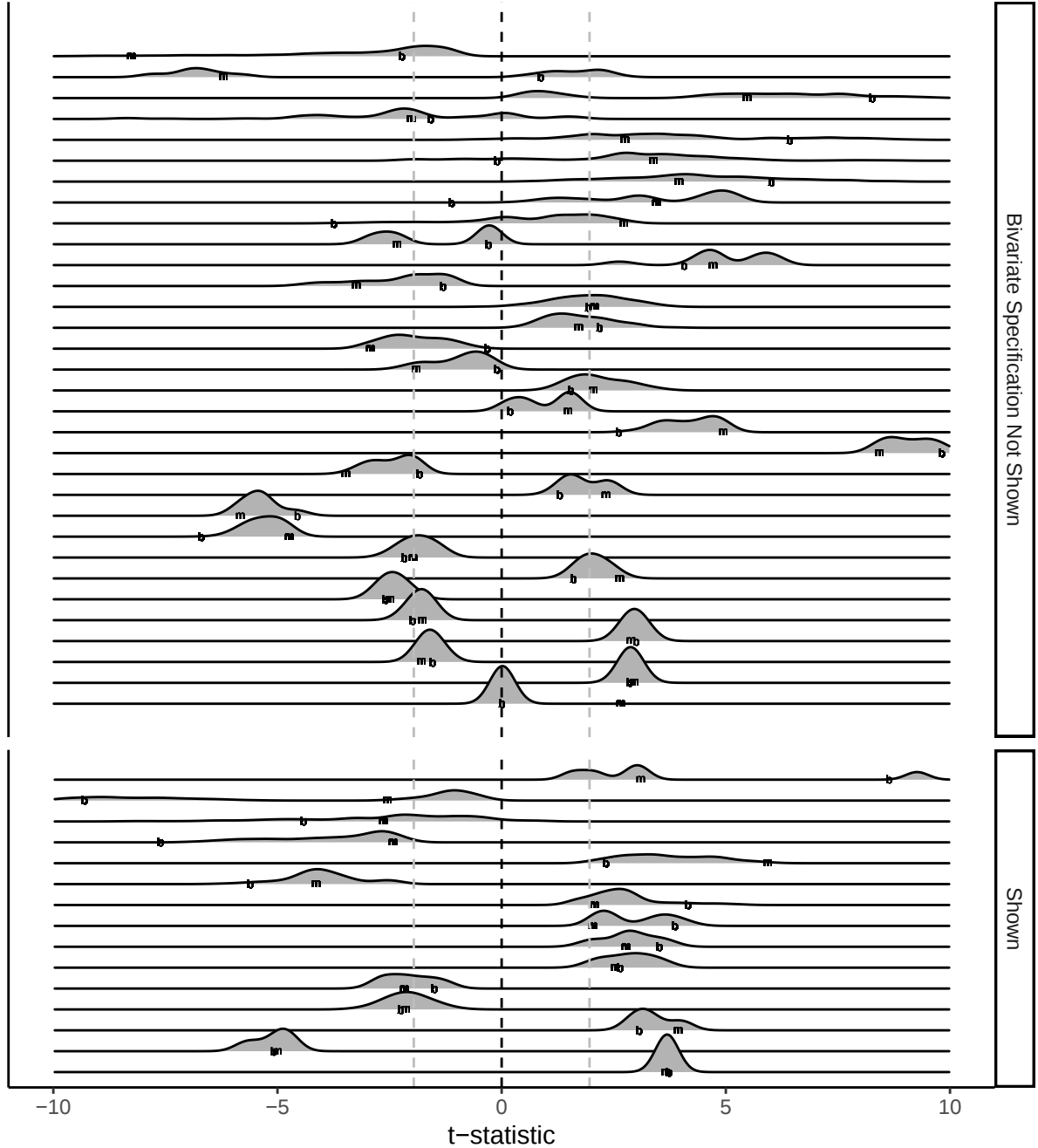
Figure 7: Distribution of t-Statistics across All Possible Control Variable Combinations for Observational Studies (randomly sampled in cases with more than 10,000 combinations, sorted by variance). ‘m’ shows the full multivariate t-statistic and ‘b’ the bivariate t-statistic. The grey dotted lines mark t-statistics at -1.96 and 1.96, the p = 0.05 thresholds for conventional statistical significance. We exclude two studies here because of the inordinate time required to estimate each specification.
